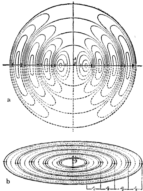
FIG. 1. THE FIELDS ABOUT A VERTICAL HERTZIAN ANTENNA
