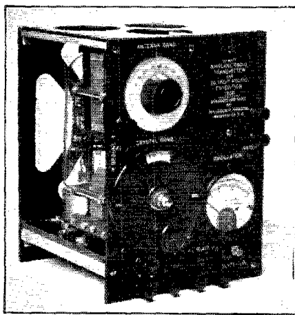
THE AIRPLANE TRANSMITTER built by Malcolm P. Hanson for the Detroit Arctic Expedition. It has a power of 50 watts, is crystal controlled, and weighs but 7 lbs. complete with tube and crystal.
