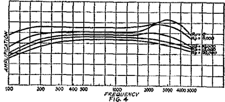
THE EFFECT OF PLATE IMPEDANCE ON THE OPERATION OF TRANSFORMER, D WHICH HAS HIGH PRIMARY IMPEDANCE
