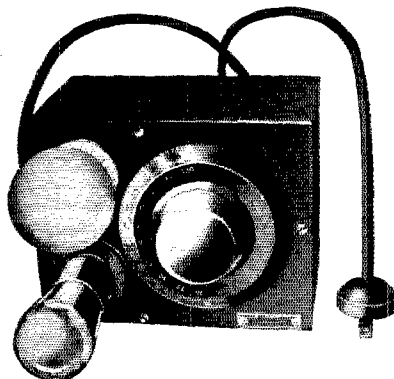
THE COMMERCIAL FORM OF THE OSCILLATOR This device is called the "Superunit set tester" and has a wavelength range of 200-575 meters. The dial carries both a wavelength scale and a 1 0-100 scale.
