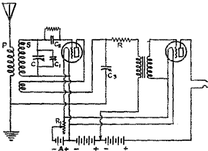
FIG. 1. THE CR-18 CIRCUIT C—Maximum of 130 \mu fd. C1—Vernier of 3 \mu fd. maximum capacity. C2—40 \mu fd. C3—226 \mu fd. R—25,000 ohms. R1—10 ohms.
