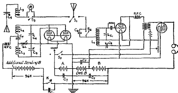
THE TRANSMITTER-RECEIVER DIAGRAM OF CONNECTIONS
