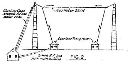
THE MULTIPLE-TUNED ANTENNA FOR THE 1560-METER STATION
