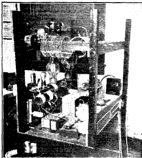
REAR VIEW OF TRANSMITTER. PLENTY OF ROOM HERE FOR ANY EXPERIMENTAL WORK
