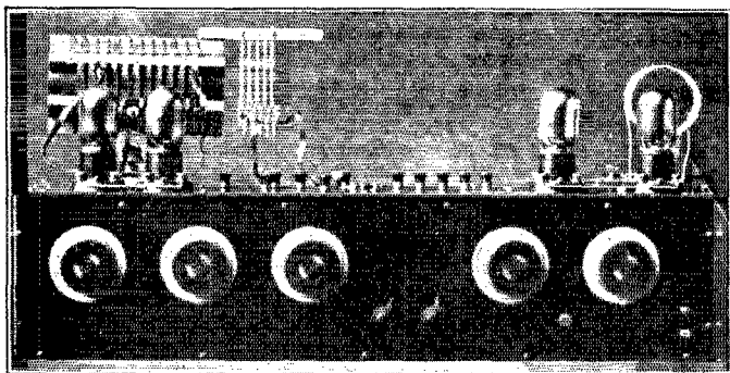
FRONT VIEW OF THE TRANSMITTER-RECEIVER
