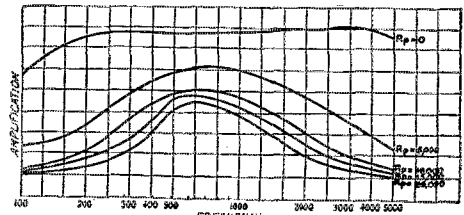
THE EFFECT OF VARYING THE PLATE IMPEDANCE OF THE PLATE WORKING INTO TRANSFORMER A, WHICH HAS A LOW PRIMARY IMPEDANCE
