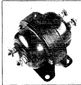
Transformer A. The familiar General Electric "distortion transformer," designed for 500-cycle spark reception or other signals giving a 1000-cycle tone. Also known as UV-712.
