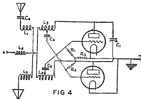
FIG 4 CIRCUIT OF 100-WATT PUSH-PULL TRANSMITTER AT 1XM
