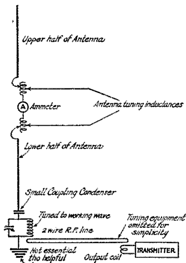
FIG 1 THE ANTENNA SYSTEM AT 2XAF
