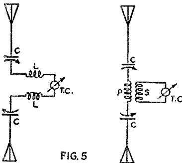
CIRCUIT OF THE EXPLORING ANTENNAS T.G. Thermo galvanometer. C.C. Tuning condensers.
