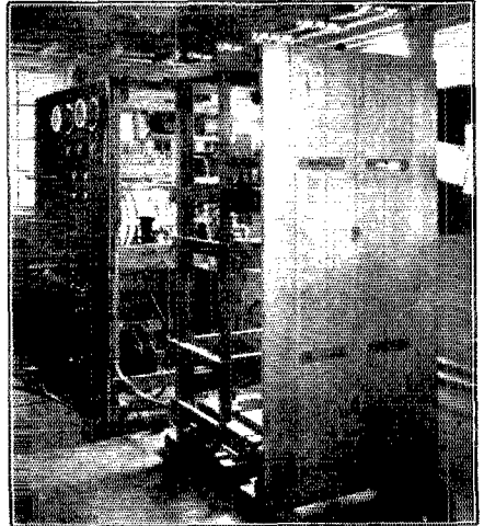
INTERMEDIATE AND FINAL STAGES OF THE 2XAF TRANSMITTER
