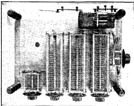
FIG. 6 BOTTOM VIEW OF STANDARD FREQUENCY TRANSMITTER SHOWING LARGE 250 \mu fd. SPECIAL NATIONAL CONDENSERS
